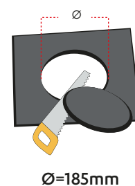
PLASTER CEILING HOLE SIZE
