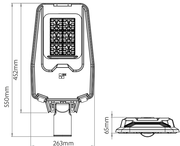
TECHNICAL DRAWING
