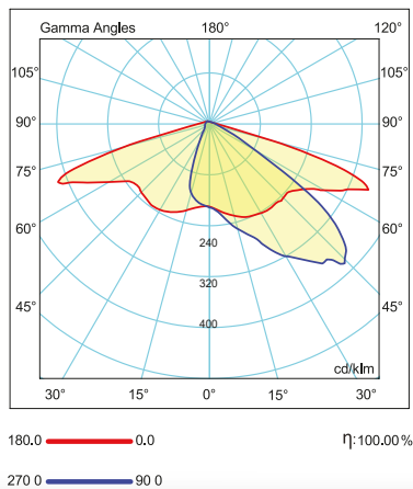
PHOTOMETRIC DISTRIBUTION
