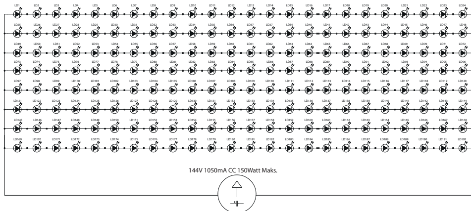
MODHEX-24S8P-104X311mm-144/700mA-1050mA/100W-150W V1.0
