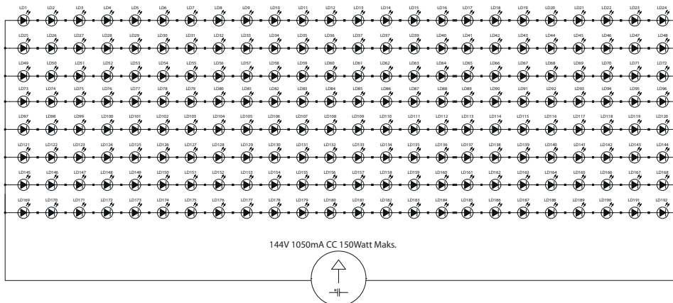
MODHEX-24S8P-104X311mm-144/700mA-1050mA/100W-150W V1.0
